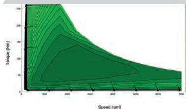
Efficiency Map % (*)
