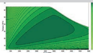
Efficiency Map % (*)
