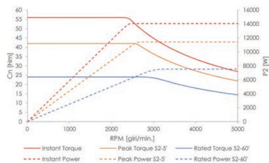
Speed- Torque & Speed Power Motor Curves
